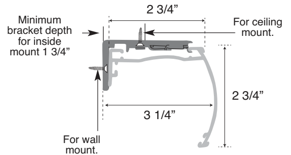
Universal ceiling or wall mount bracket
